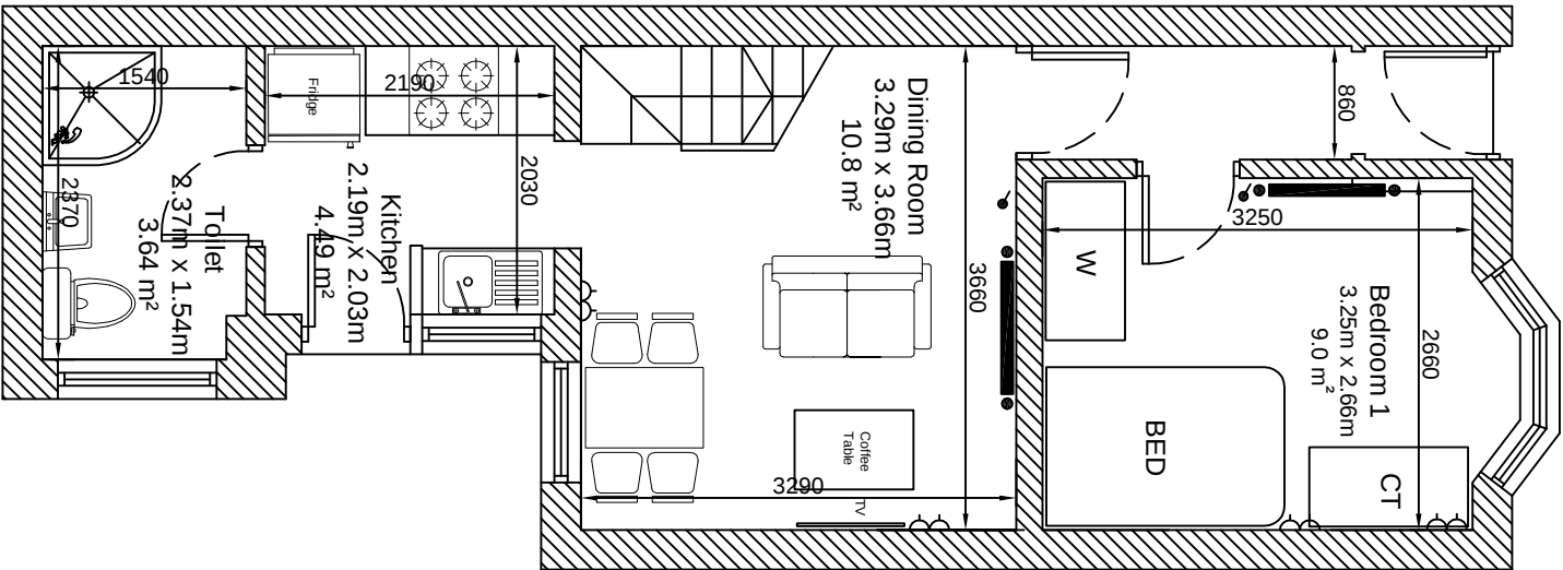
PROPOSED GROUND FLOOR GROSS INTERNAL FLOOR AREA 33.9 SQ M
